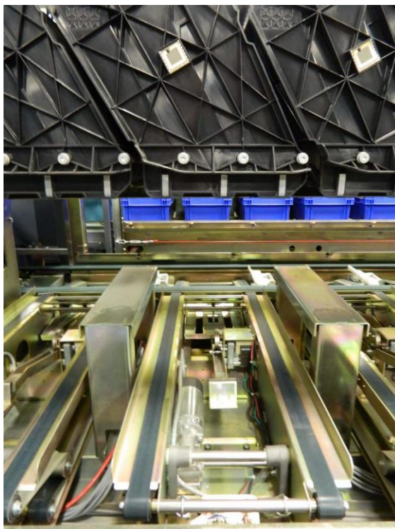
Defs.' Mot. Ex. 14 (photograph of place-and-transfer device).
