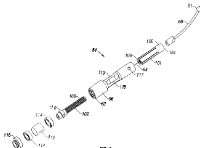
FIG. 5 Lead Screw Assembly
